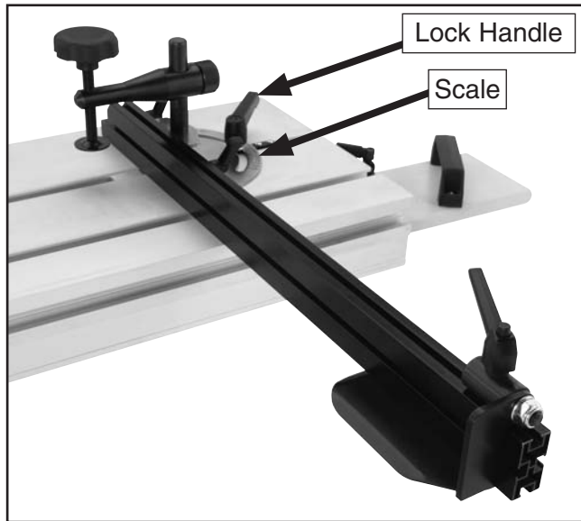
Figure 63. Miter fence.
